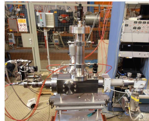
BSM Proton linac
