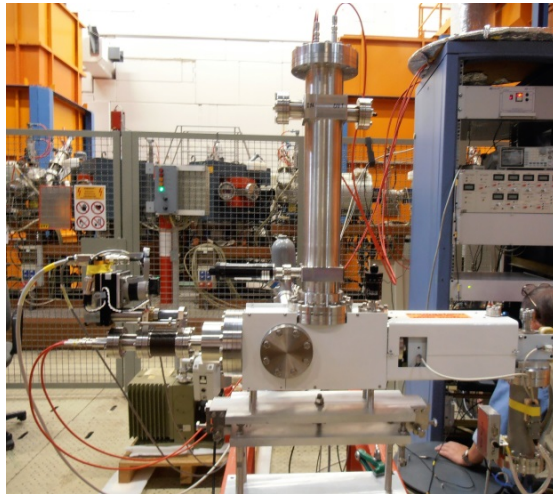
BSM UNILAC
